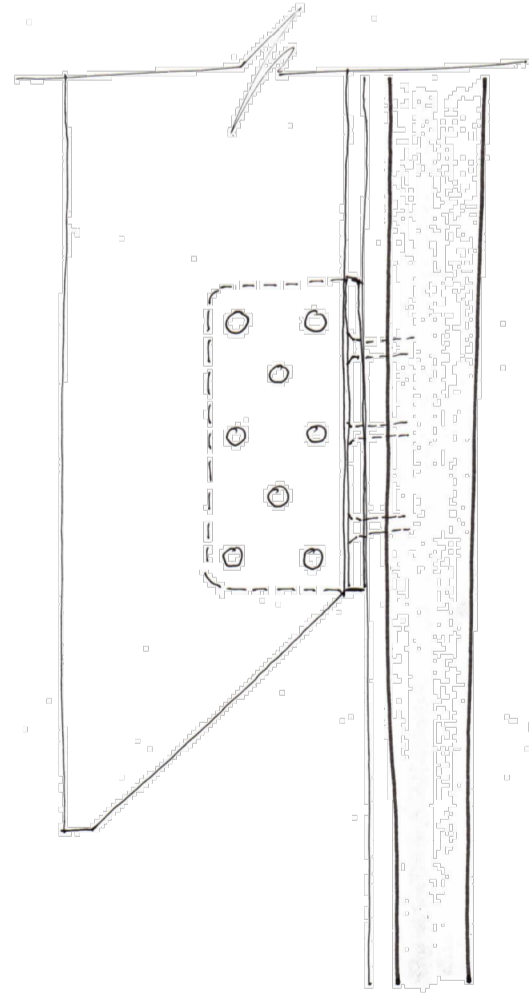
SKETCH DETAILS
